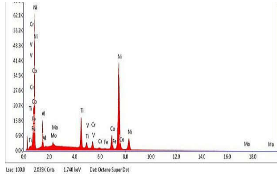
Fig. 16. EDS spectrum of selected area 1
