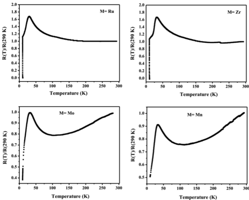
Fig. 4. Normalized resistance as a function of temperature of the \text{Ru}_{0.9}\text{M}_{0.1}\text{Sr}_2\text{GdCu}_2\text{O}_8 system, with M = \text{Ru}, \text{Zr} , and Mn.
