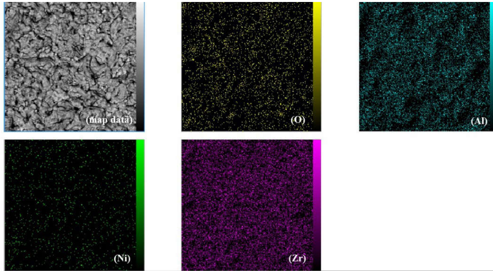
Fig. 8. X-ray map of the elements of the surface of AHZ30 sample after 120 h cyclic oxidation at 1000°C.
