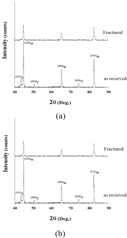
Fig. 5. X-ray diffraction patterns of microstructures of the as-received and uniaxially deformed state (fractured) TRIP800 steels: (a) TRIP1 (b) TRIP2.
