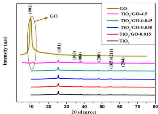
Fig. 1. X-ray diffraction patterns of TiO 2 , TiO 2 /GO-0.015, TiO 2 /GO-0.030, TiO 2 /GO-0.045, TiO 2 /GO-4.5 thin films and graphene oxide (GO) nanopowders.
