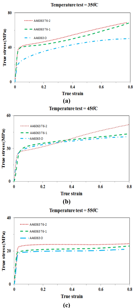
Fig. 11. True stress-true strain curves of AA6063 T6-2, AA6063 T6-1, and AA6063 O during hot deformation at \dot{\epsilon}=0.1\text{ s}^{-1} and different temperatures of (a) 350, (b) 450, and (c) 550°C.
