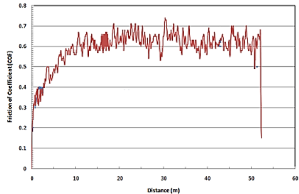
Fig. 10. Changes in wear in the friction coefficient of the reference sample in wear under a load of 300 g force and a distance of 50 m.
