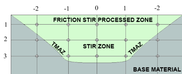
Fig. 2. Microhardness
