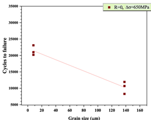
Fig. 15. increasement of fatigue life due to reduction of grain size
