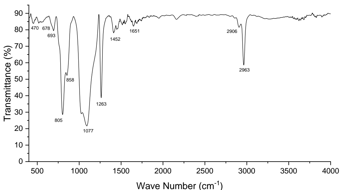
Fig. 6. FTIR peaks of a hybrid of \text{SiO}_2 - \text{TiO}_2 gels
