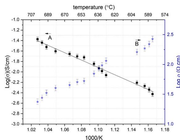
Fig. 4. The measured ionic conductivity of the molten glass B_{82.5}O_{17.5} , which nominally contained 17.5Li 2 O + 82B 2 O 3 (mol%) with temperature. curve (A) shows the conductivity as a function of temperature, where the experimental errors are evolving. The data in the curve (B) are the logarithmic specific resistivity with temperature
