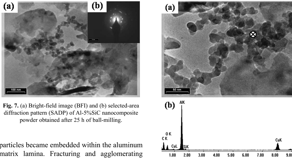
Fig. 8. (a) BFI of Al-5%SiC nanocomposite powder obtained after 25 h of ball-milling and (b) EDS analysis of the region marked in (a).
