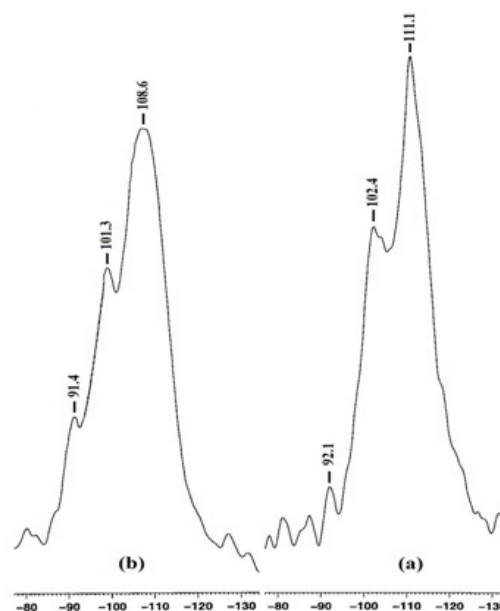
Fig. 2. \text{Si}^{29} MAS-NMR spectra of the gel powder (a) without carbon phase and (b) with carbon phase
