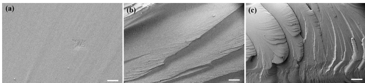
Fig. 8. Fracture surface of different specimens: EC0 (a), EC6 (b), and EC3. Scale bars in the image are 10 \mu\text{m} .
