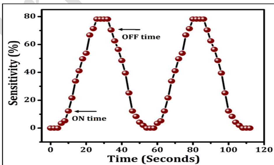
Fig.13. Response and recovery time.
