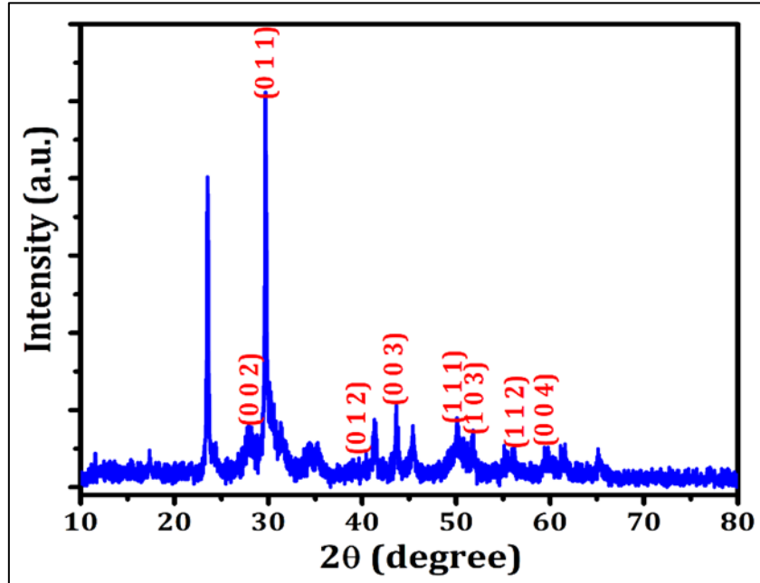
Fig. 3. XRD pattern of ZrSe_2 thick films.
