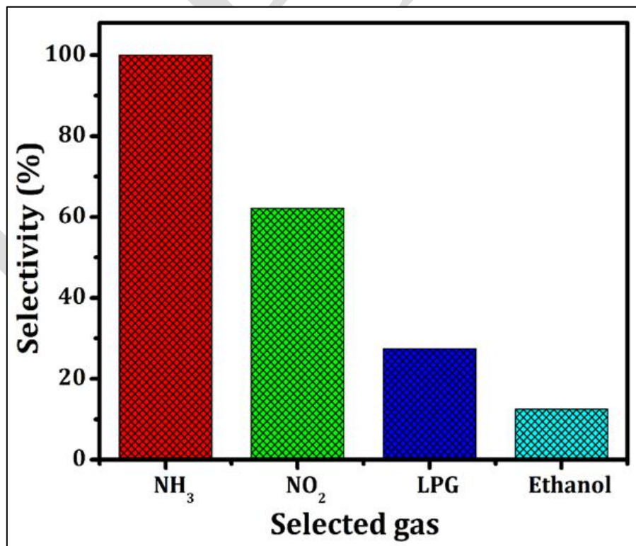
Fig.11. Selectivity plot
