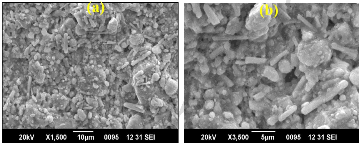
Fig. 6. (a-b) SEM micrograph of ZrSe_2 thick film.
