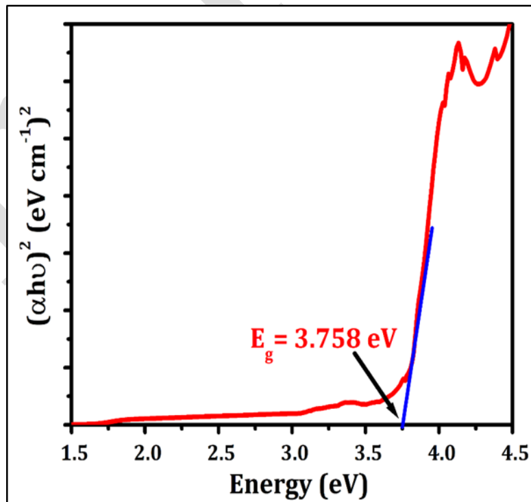
Fig.5. Plot of (\alpha h\nu)^2 versus (h\nu) for \text{ZrSe}_2 thick film.
