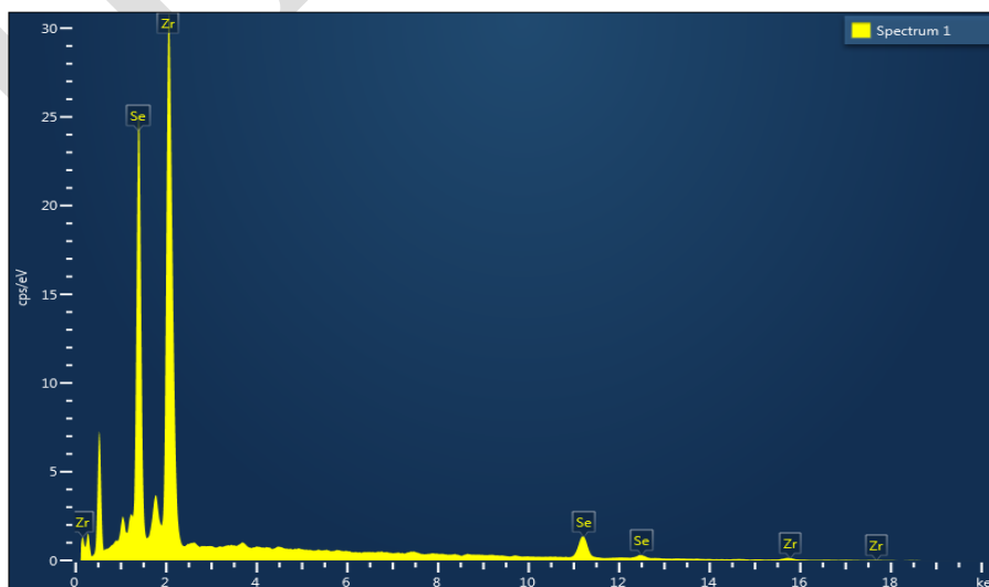
Fig.7. EDX pattern of ZrSe_2 thick films.
