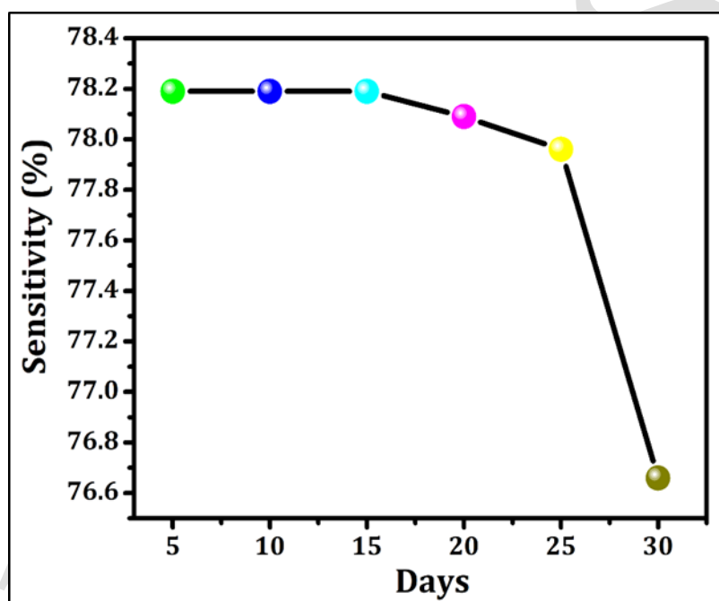
Fig.14.Reusability of ZrSe 2 thick film.
