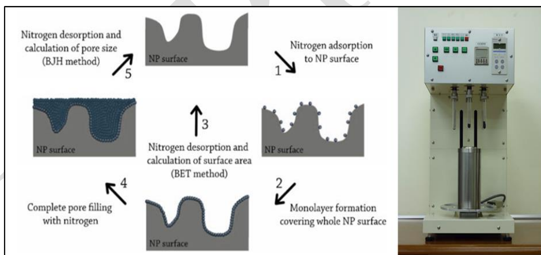
Fig. 2. Schematic of BET method apparatus
