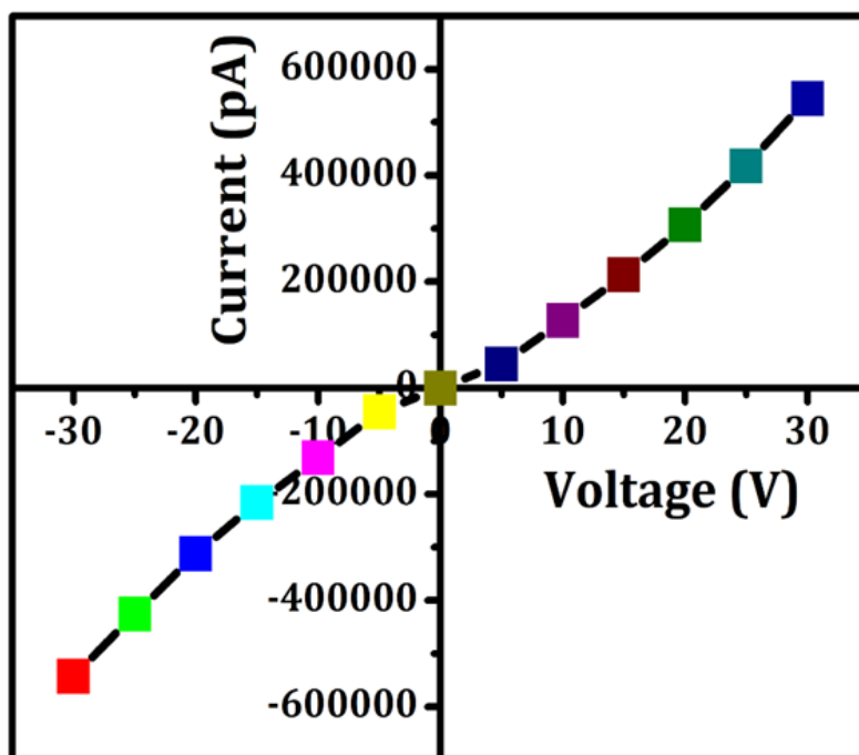
Fig. 8. I-V characteristics
