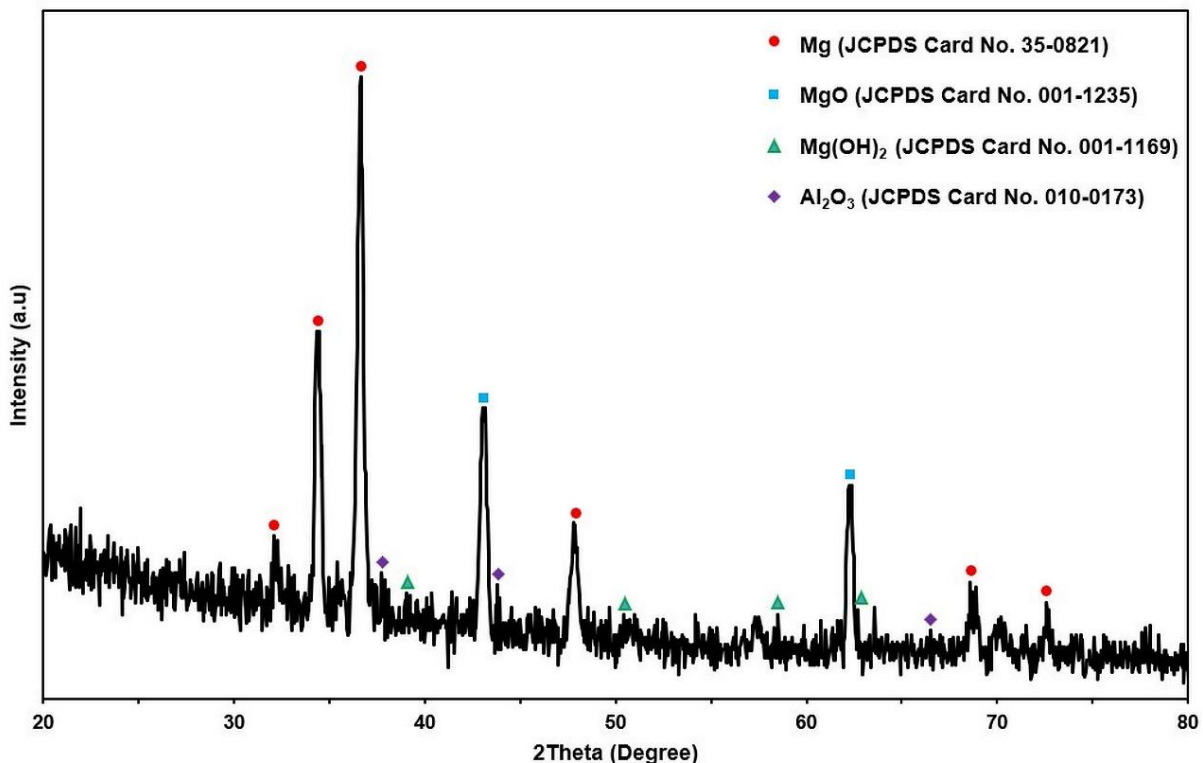
Fig. 8. XRD diffractogram of an anodized surface
