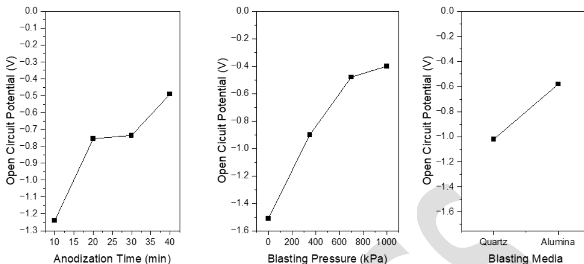
Fig. 13. Main effects plot for OCP
