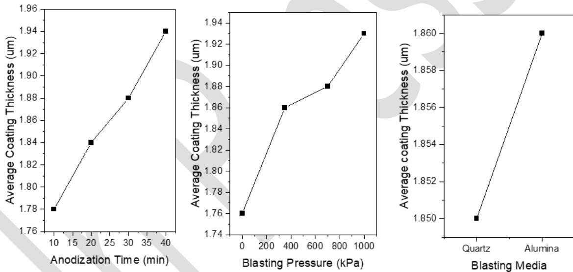
Fig. 11. Main effects plot for coating thickness
