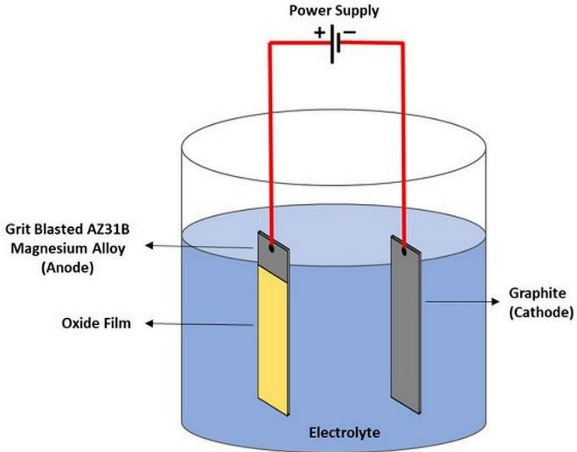
Fig. 1. Schematic diagram of anodizing process utilized in this study
