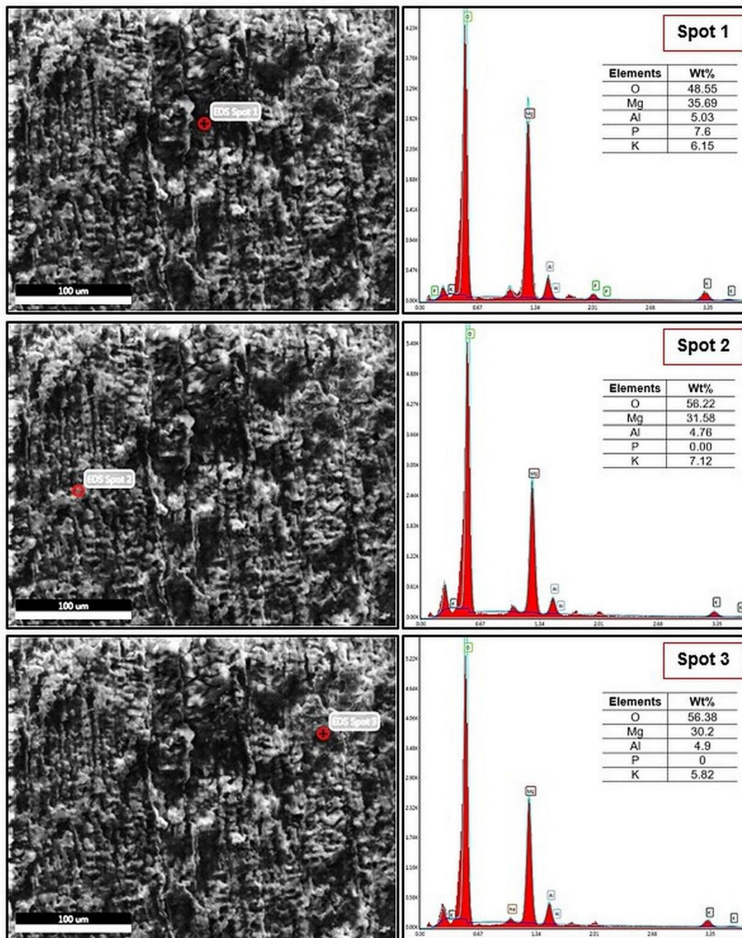
Fig. 6. EDX analysis of an anodized surface
