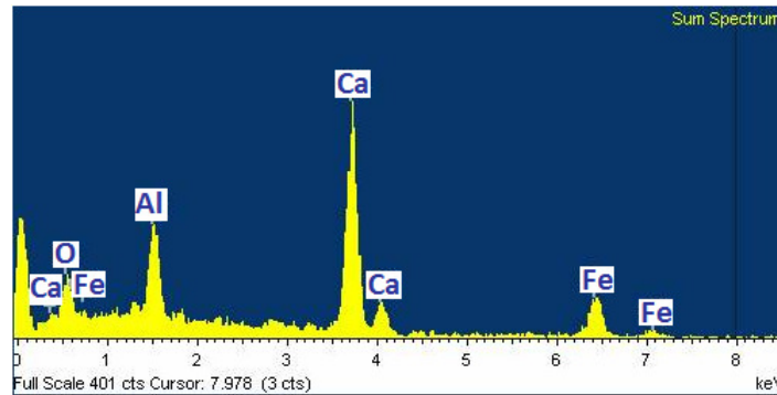
Fig. 7. EDS analyses of region GB (grain boundaries) in Fig. 6-b.
