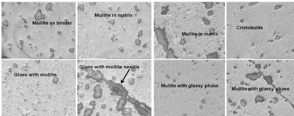
Fig. 9 (a) Microscopic studies of the bricks made from feed samples
