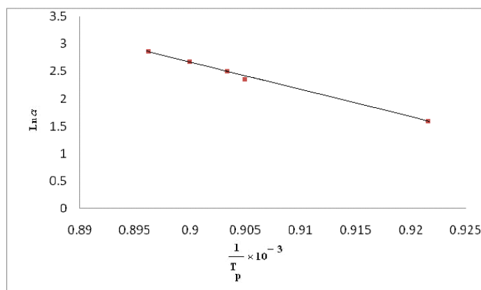
Fig 8. Variation of \text{Ln } \alpha vs \frac{1}{T_p} in \text{ST}_3\text{Z}_1\text{Y}_1 for determination of the crystallization activation energy according to Marotta method
