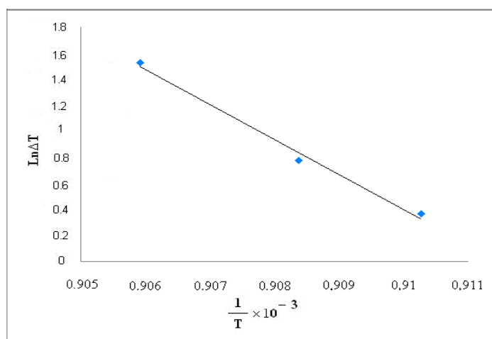
Fig 9. Variation of \text{Ln } \Delta T vs \frac{1}{T} in \text{ST}_3\text{ZY}_1 for determination of the Avrami exponent according to Marotta method
