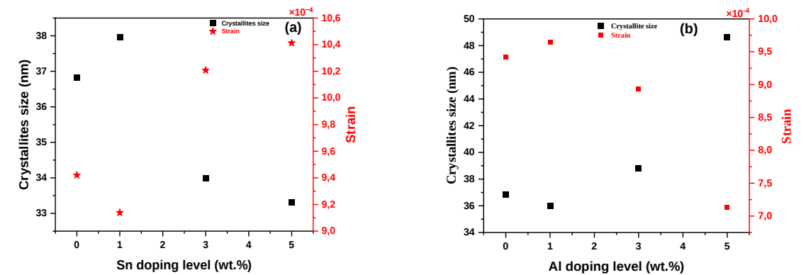
Fig. 5. Effect of a) Sn and b) Al doping concentrations on crystallite size and microstrain in ZnO thin films, calculated using Scherrer's equation
