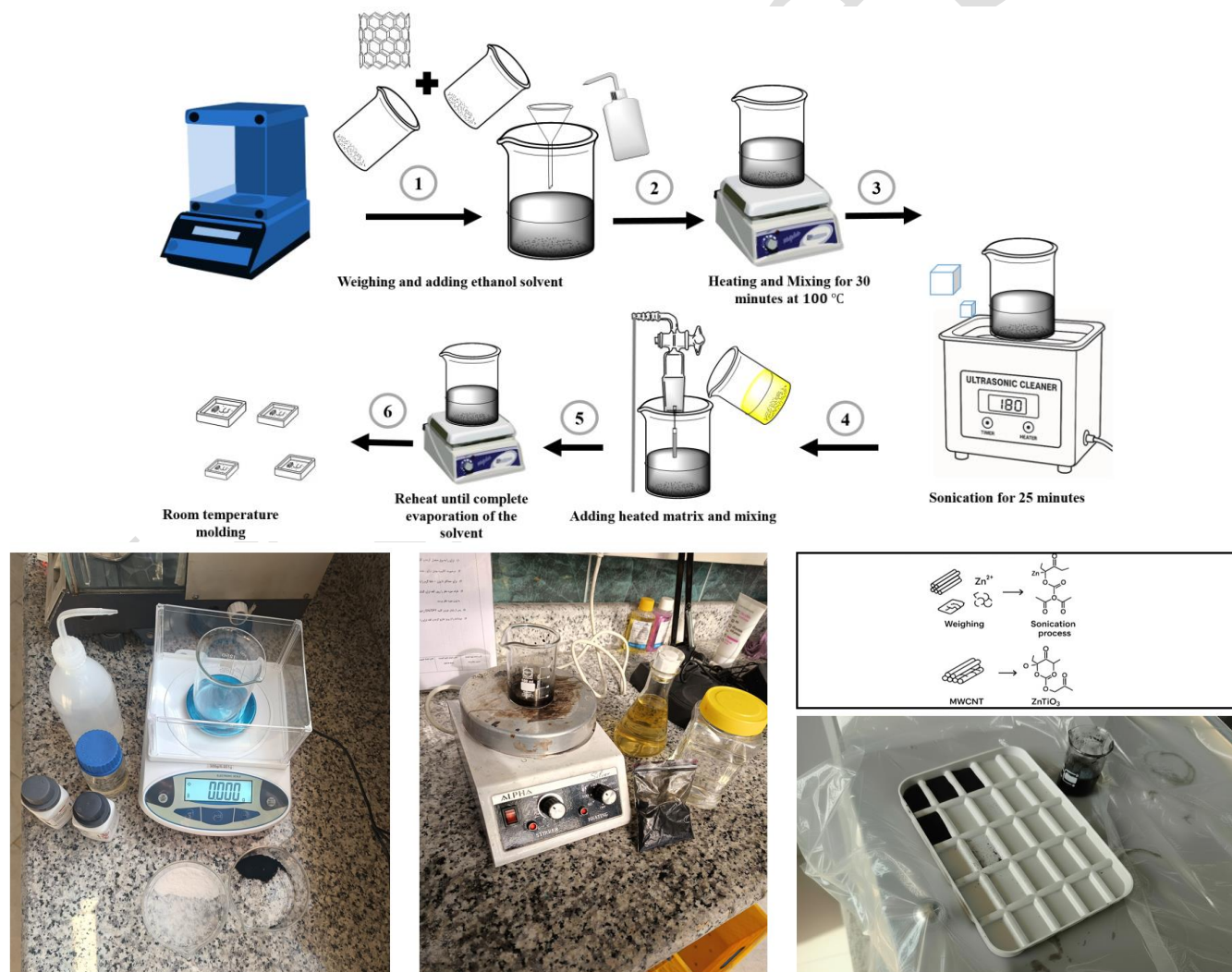
Fig. 4. Experimental procedure for laboratory-scale nanocomposite fabrication
