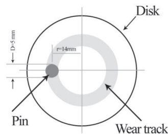
Fig. 2. Schematic of pin-on-disk configuration.
