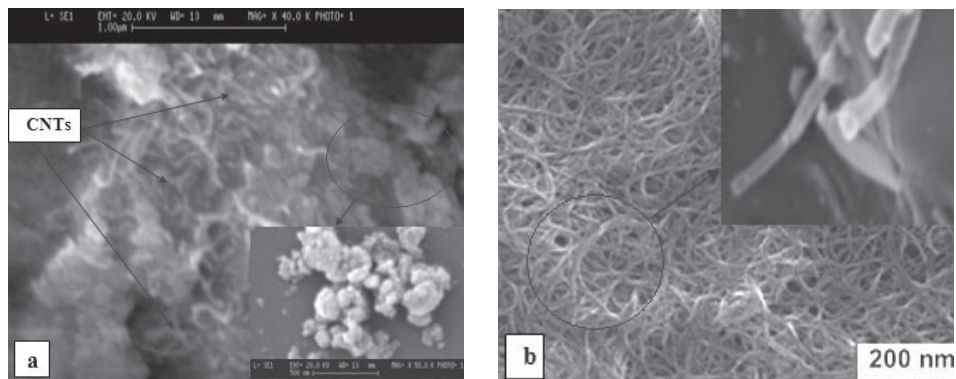
Fig. 5. SEM micrographs of synthesized HAp -CNTs powders at different magnifications
