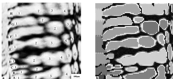
Fig. 5. SEM images of the stirred alloys cooled to two-phase region: (a) Cooled to 610 °C, sheared at 1000 S -1 for 20 seconds, after isothermal holding for 80 sec, WQ and (b) COM of (a).
