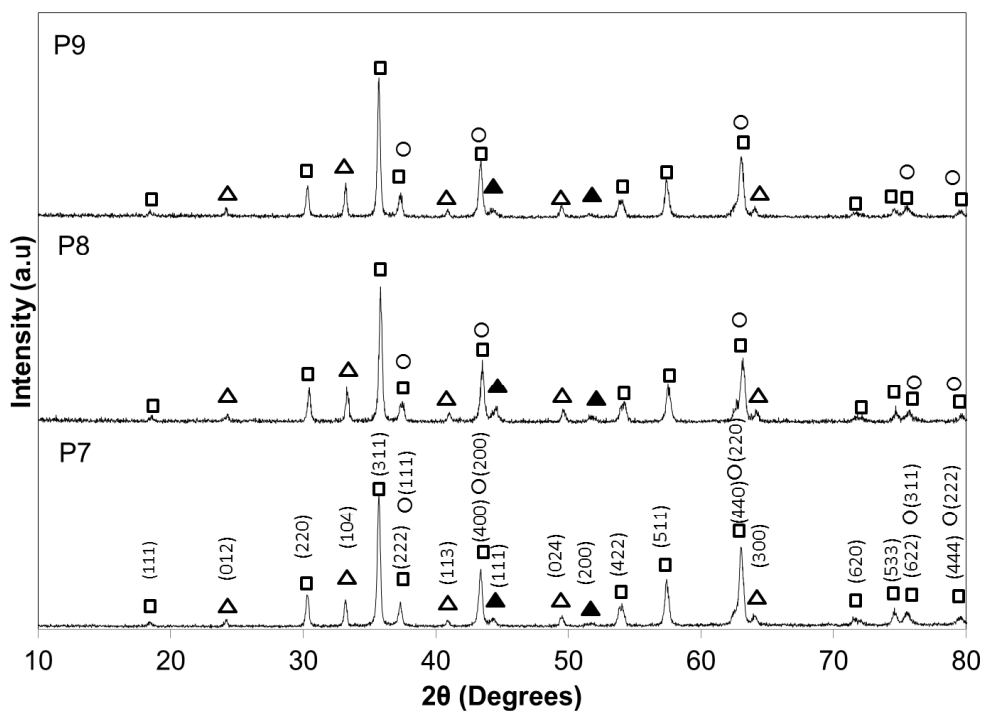
Fig. 1. XRD patterns of the combustion products for samples p7, p8 and p9. \square : \text{NiFe}_2\text{O}_4 , \Delta : \alpha\text{-Fe}_2\text{O}_3 , \blacktriangle : \text{FeNi}_3 , \circ : \text{NiO} .
