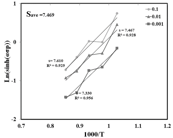
Fig. 8- The relationship between ln[sinh(ασ)]-1000/T.
