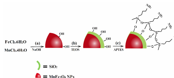
Fig. 2. Schematic illustration of \text{MnFe}_2\text{O}_4@SiO_2-NH_2 nanocomposite particles preparation: (a) synthesis of \text{MnFe}_2\text{O}_4 NPs, (b) formation of \text{SiO}_2 shell, and (c) synthesis of \text{MnFe}_2\text{O}_4@SiO_2-NH_2 NPs
