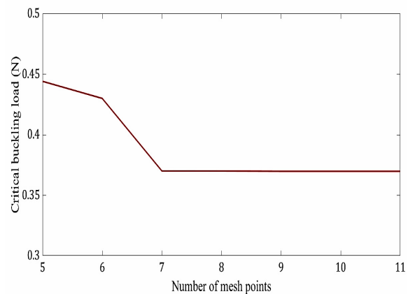
Fig. 2. The critical buckling load in terms of number of mesh point
