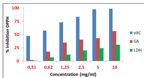
Fig. 10. The percentage (%) inhibition activity of DPPH
