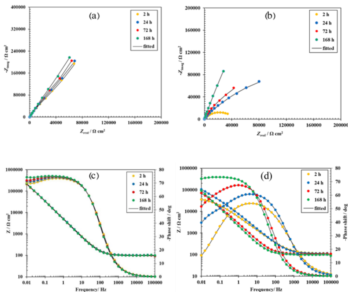
Fig. 9. Nyquist and Bode curves for coatings: (a and c) CrN, (b and d) CrN/Cu.
