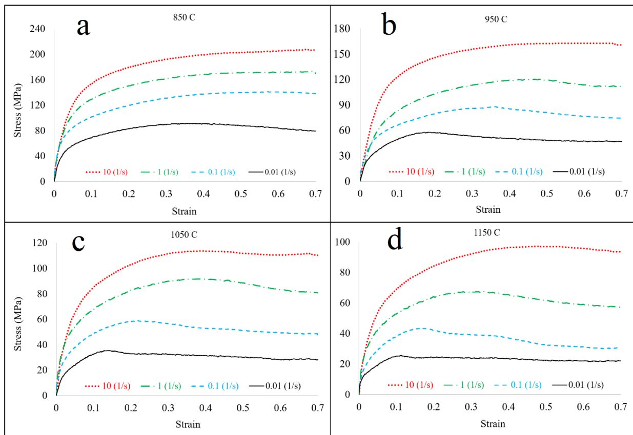
Figure 3: Stress-strain curve of compression test at temperatures a-850 °C, b-950 °C, c-1050 °C and d-1150 °C at different strain rates.
